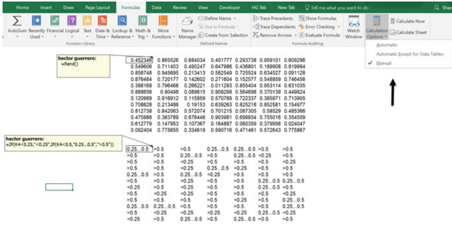
Fig. 8.3 Control of worksheet recalculation
