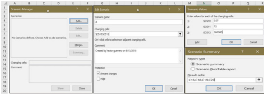
Fig. 9.15 Creating scenarios
